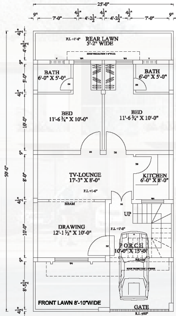
GROUND FLOOR PLAN SCALE 1/8"=1'-0" 965 sqft
